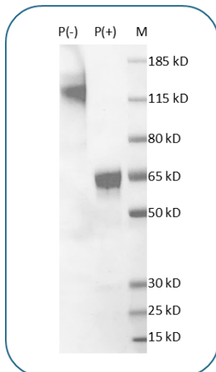
Purified Human OX40 Protein (C-Fc) on SDS-PAGE under reducing (P+) and non-reducing (P-) conditions. The purity of the purified protein appears to be greater than 95% based on reducing condition.
