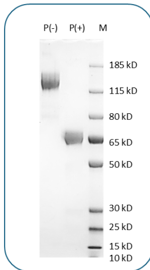
Purified Cynomolgus Monkey OX40 Protein (C-Fc) on SDS-PAGE under reducing (P+) and non-reducing (P-) conditions. The purity of the purified protein appears to be greater than 95% based on reducing condition.
